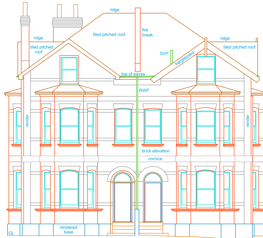
NORTH ELEVATION
